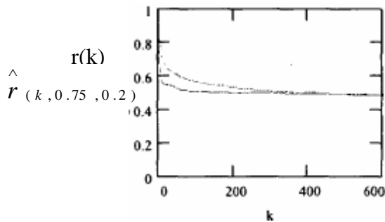
Fig. 2 Matching \hat{r}(k,0.75,0.2) with exactly self-similar Model.
