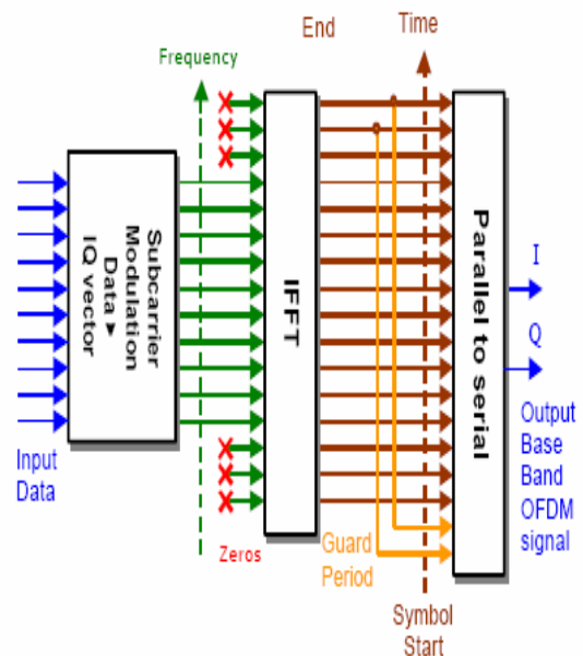
Figure 1: Generation of OFDM System
