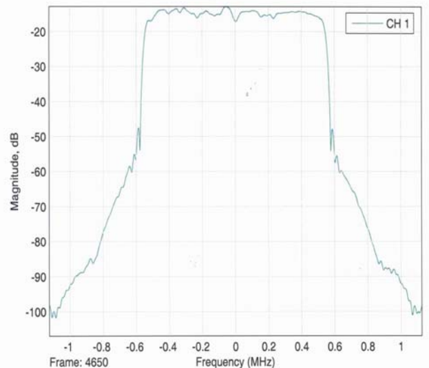
Figure 8: The received signal power spectrum after filtering
