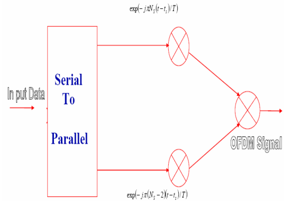
Figure2: OFDM modulator
