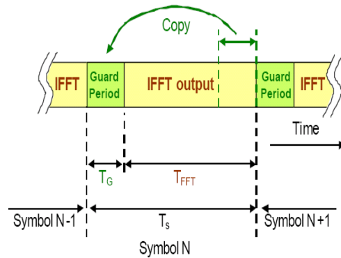
Figure 5: Addition of a guard period to an OFDM signal
