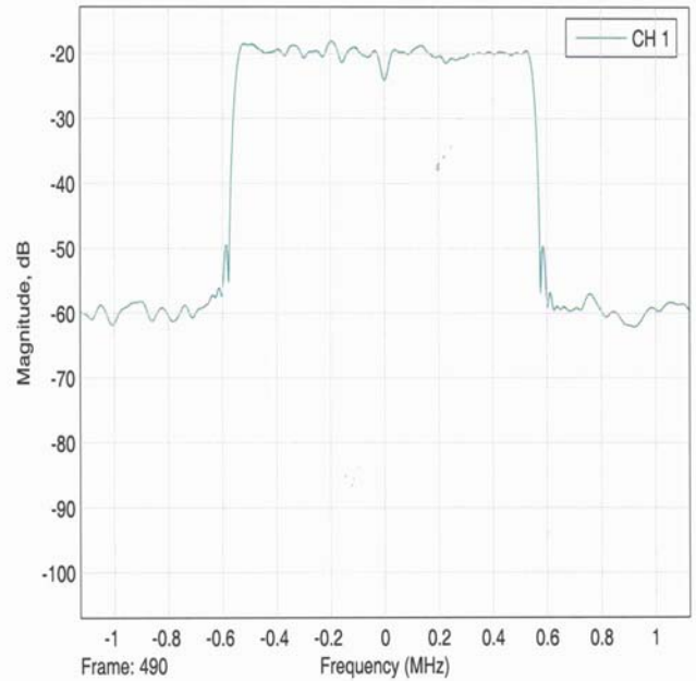
Figure7: The received signal power spectrum before filtering
